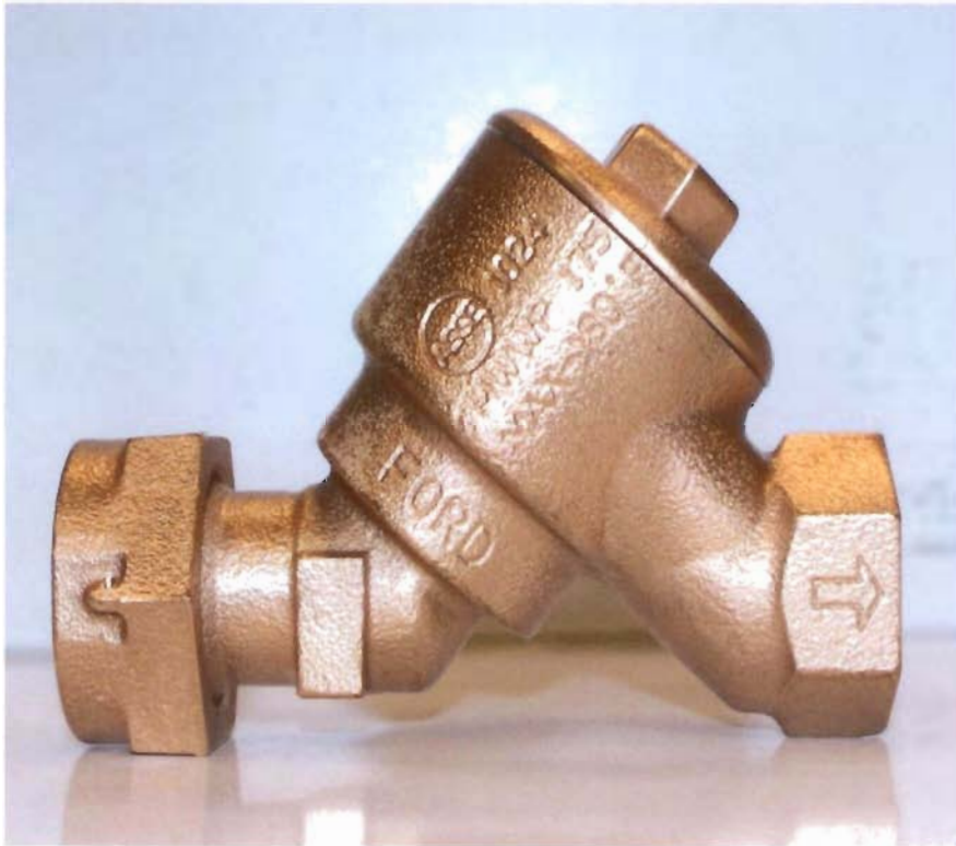
FIGURE 5 DUAL CHECK DEVICE
