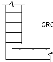
BOTTOM SLABS TO WALL
