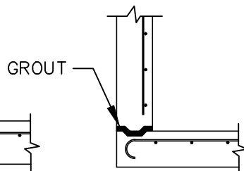
BOTTOM SLABS TO WALL
