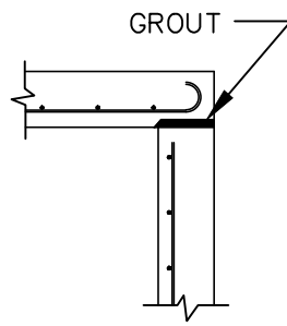
TOP SLABS TO WALL
