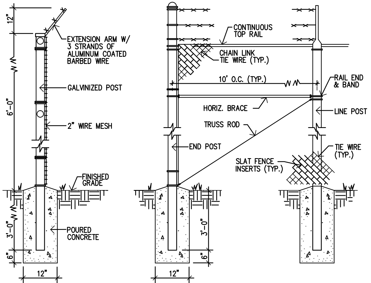
TYPICAL FENCE POST
