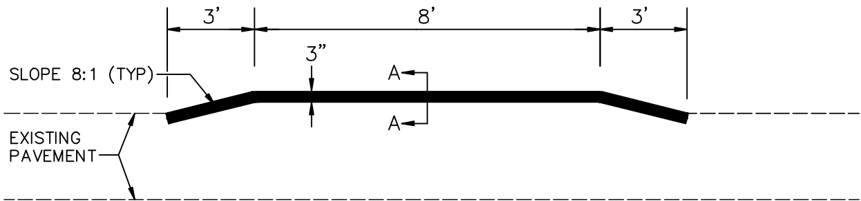
PROFILE VIEW
