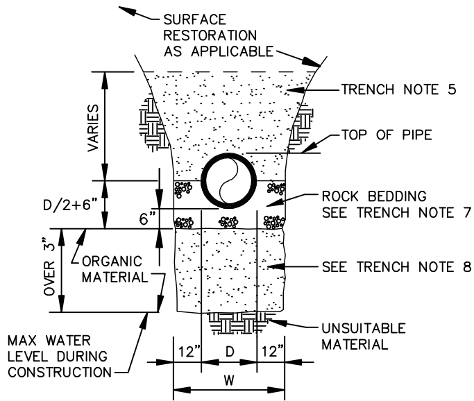
TRENCH BACKFILL / BEDDING CLASS " D "
