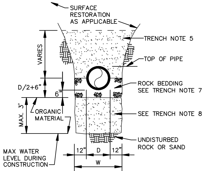
TRENCH BACKFILL / BEDDING CLASS " C "
